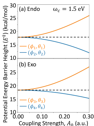
Figure 5. Polaritonic ground state activation energy, defined as the energy difference between the transition state and the reactant geometries, E^\ddagger = E_0(\mathbf{R}_{\text{TS}}) - E_0(\mathbf{R}_{\text{reac}}) , for the two reaction pathways, (a) Endo and (b) Exo. The cavity polarizations are shown at the critical points for each pathway: (\phi_1, \theta_1) and (\phi_3, \theta_3) (MAX in orange); (\phi_2, \theta_2) and (\phi_4, \theta_4) (MIN in blue). The cavity frequency is \omega_c = 1.5 eV. The horizontal dashed line indicates the uncoupled barrier height (i.e., A_0 = 0.0 au).
