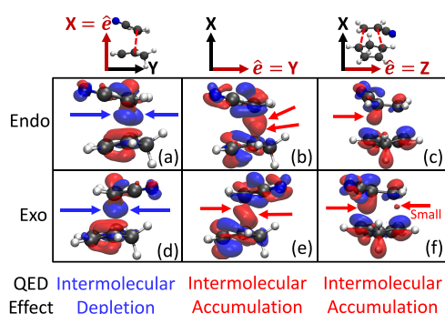
Figure 3. Difference density isosurfaces of the transition state geometries for the (a–c) Endo and (d–f) Exo pathways. The cavity polarization direction is along the (a, d) X -, (b, e) Y -, and (c, f) Z -directions. The isosurfaces in each panel correspond to the difference density, \Delta\rho_{00}(x, y, z) = \rho_{00}^M(x, y, z) - \xi_{00}(x, y, z) , at the transition state geometry using the pQED-TDDFT approach of the current work. The color indicates the accumulation (red) or depletion (blue) of electron density upon coupling to the cavity. The arrows indicate the corresponding change of electron density that can be interpreted as “intermolecular bonding orbitals”. In all cases, the light-matter coupling strength A_0 = 0.2 au with cavity frequency \omega_c = 1.5 eV. The isovalue chosen for the X -direction is 1.0 and 0.2 m\text{el}/\text{\AA}^2 for the Y - and Z -polarizations, where m\text{el} = |e| \times 1000 and |e| is the charge of an electron.
