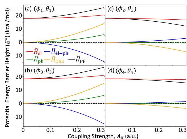
Figure 8. Energy contributions from individual terms from \hat{H}_{\text{PF}} in eq 1 to the ground state energy barrier height for each of the four extrema points (a–d) defined as white circles in Figure 4. Components are \hat{H}_{\text{el}} in red, \hat{H}_{\text{el-ph}} in blue, \hat{H}_{\text{ph}} in green and \hat{H}_{\text{DSE}} in gold. The horizontal dashed black line indicates the barrier height changes outside the cavity (i.e., A_0 = 0.0 au). The cavity frequency is \omega_c = 1.5 eV.
