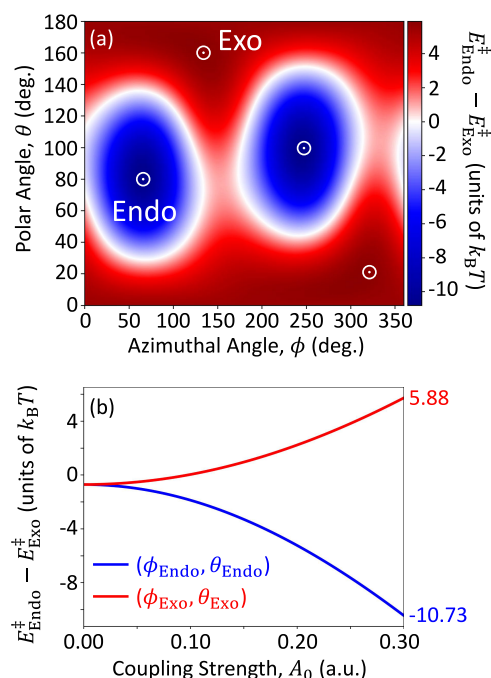
Figure 7. (a) TS energy difference between the Endo and Exo isomers, E_{\text{Endo}}^{\ddagger} - E_{\text{Exo}}^{\ddagger} , as a function of the cavity polarization direction, ( \phi, \theta ). The blue region ( E_{\text{Endo}}^{\ddagger} < E_{\text{Exo}}^{\ddagger} ) indicates that the Endo pathway has a lower barrier energy and is preferable compared to the Exo pathway; the red region, in contrast, indicates that the Exo pathway is preferable. The light-matter coupling strength A_0 = 0.3 au and the cavity frequency \omega_c = 1.5 eV. The white circle-dot symbols indicate the critical points at which E_{\text{Endo}}^{\ddagger} - E_{\text{Exo}}^{\ddagger} is maximized, (\phi_{\text{Exo}}, \theta_{\text{Exo}}) = (137.5^\circ, 160.4^\circ) , or minimized, (\phi_{\text{Endo}}, \theta_{\text{Endo}}) = (68.8^\circ, 80.2^\circ) , offering the maximum amount of selectivity for the Exo and Endo isomers, respectively. (b) TS barrier energy difference between the Endo and Exo isomers, E_{\text{Endo}}^{\ddagger} - E_{\text{Exo}}^{\ddagger} , as a function of the light-matter coupling strength at the critical angles which produce the maximal selectivity of Endo (blue) and Exo (red) isomers.
