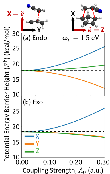
Figure 1. Polaritonic ground state activation energy, defined as the energy difference between the transition state and the reactant geometries, E^{\ddagger} = E_0(\mathbf{R}_{\text{TS}}) - E_0(\mathbf{R}_{\text{react}}) , for the two reaction pathways, (a) Endo and (b) Exo. Here, E_0(\mathbf{R}) is the polaritonic ground state energy defined in eq 3 at nuclear geometry \mathbf{R} . The colors correspond to cavity polarizations along the X- (blue), Y- (orange), and Z- directions (green). The cavity frequency is \omega_c = 1.5 eV. The horizontal dashed line indicates the uncoupled barrier height ( i.e. , A_0 = 0.0 au).
